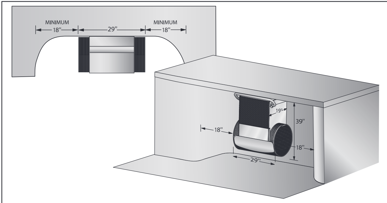
Fig. 2.1 Minimum Clearance Guide
