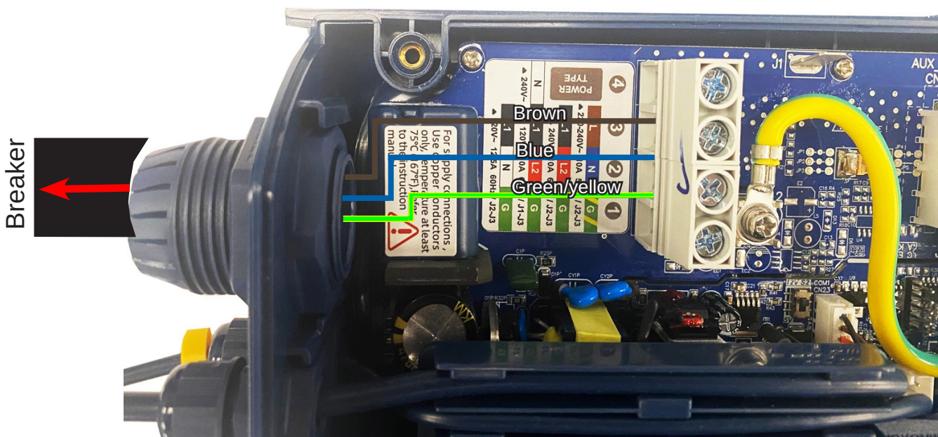
Control Box
