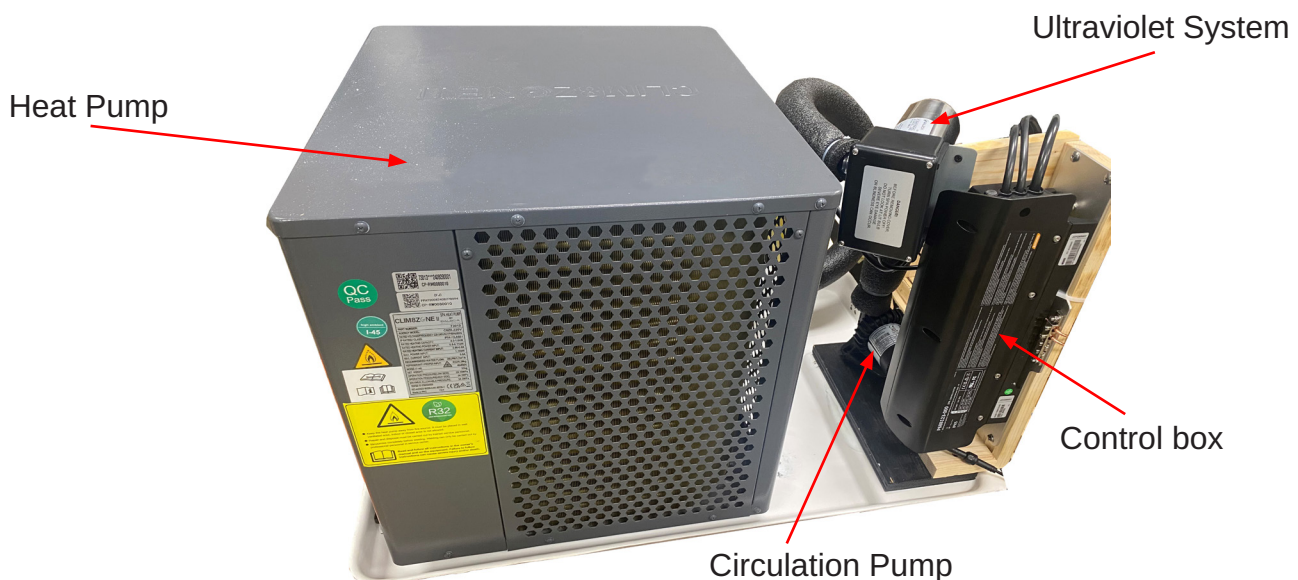
Electrical Components inside Equipment Compartment
