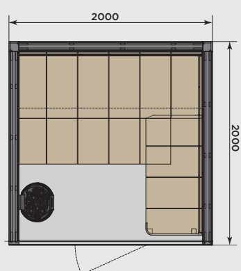
SHV2020
