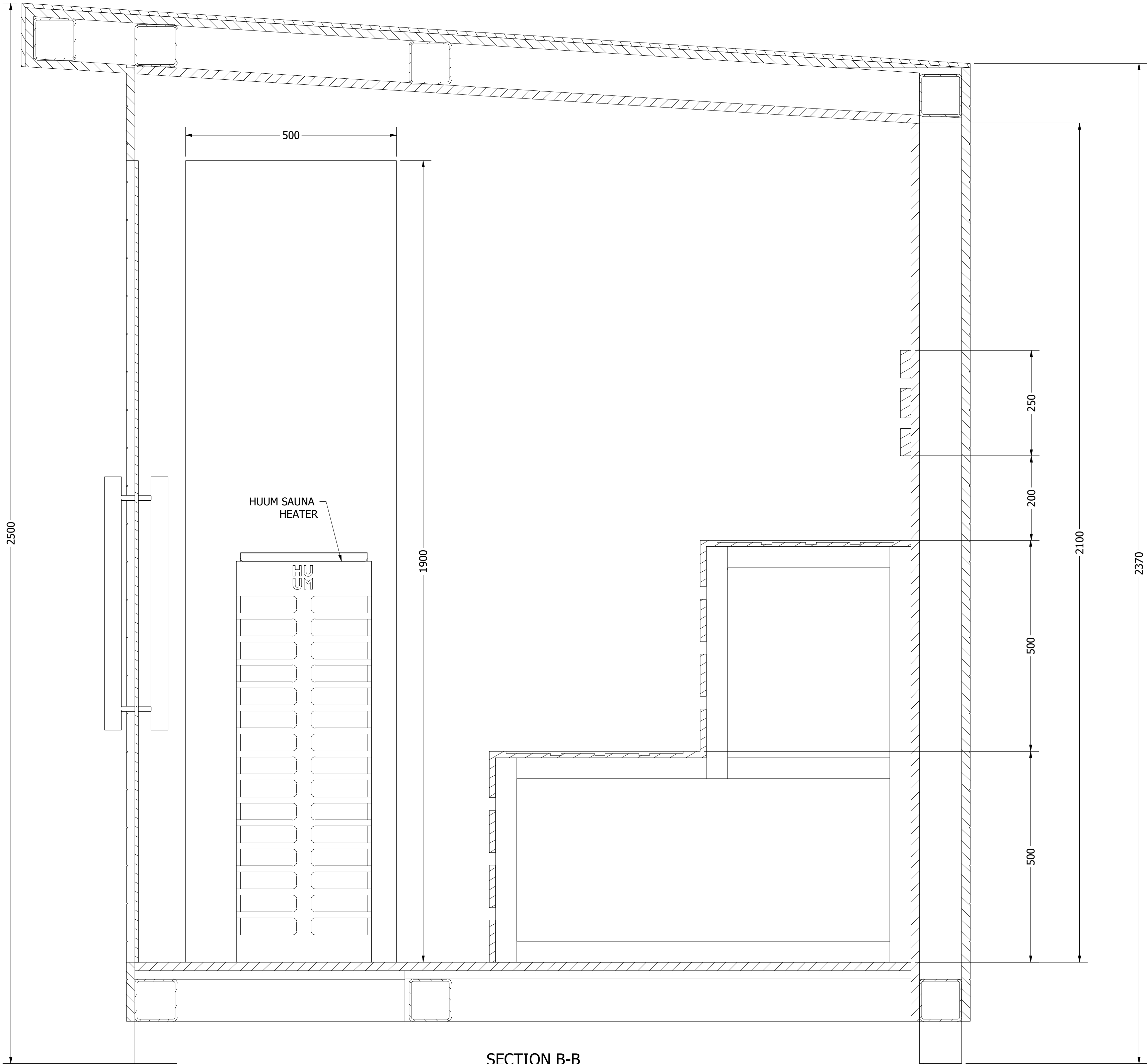
SECTION B-B SCALE 1 / 6
