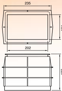
Parallel Extension Throat
