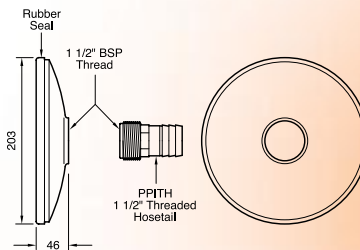
HD103 Accessory to Skimmer for Vacuuming Pool
