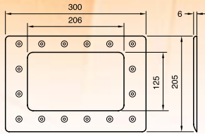
Front Finishing Plate Pt No 419N
