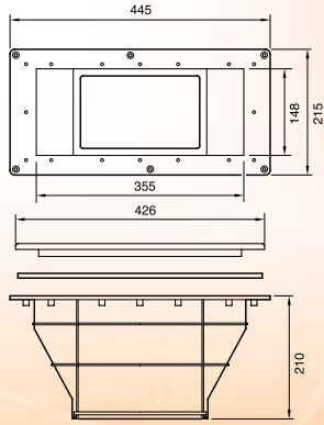
HD101CS Conc. HD101LS Liner
