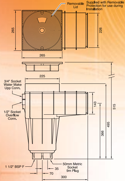
HD100NS (conc/collar) HD100N (conc/flap) HD100LAK (Liner adapt. kit)
