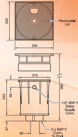
HD108 Water Level Controller Comes Complete with Float Operated Valve.
