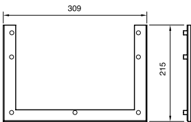
Clamp Plate Pt No 418N
