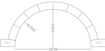
5ft Roman End Bay *Finished wall to wall measurements
