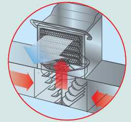
ORIGINAL ENDLESS POOL SINGLE PROPELLER, 5 HP SYSTEM
