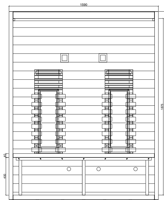
Back Panel
