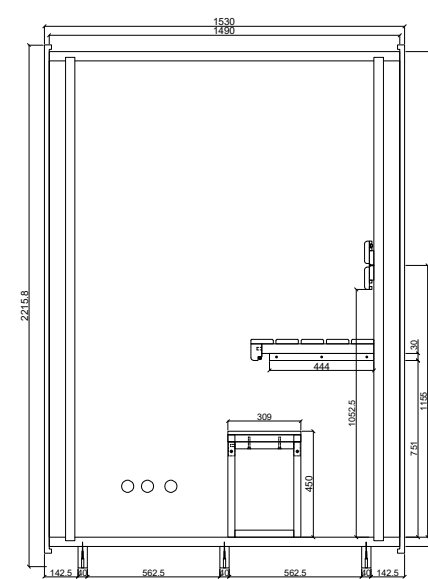
Section view
