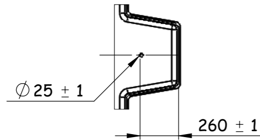
DETAIL C SCALE 1 : 25
