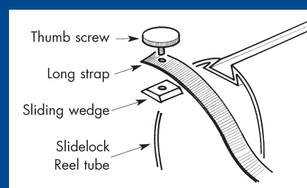
Strap fixing assembly
