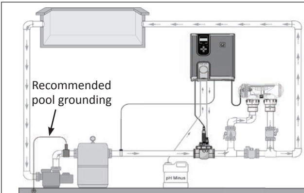
In-line installation
