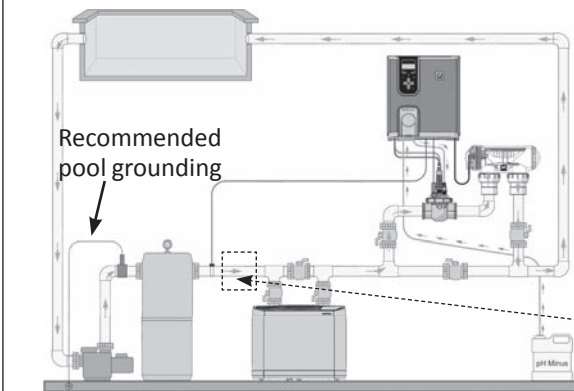
Installation with a heating system
