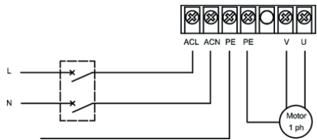
Fig 3: Terminal connections within the inverter.
